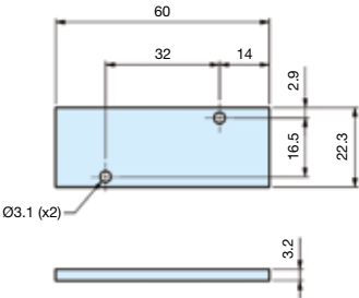
Blanking plate for manifold bar, P2LB
